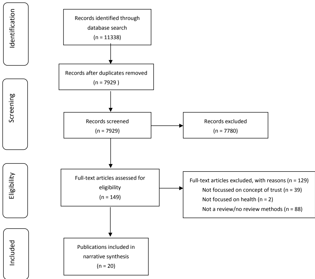
Figure 3: PRISMA diagram
